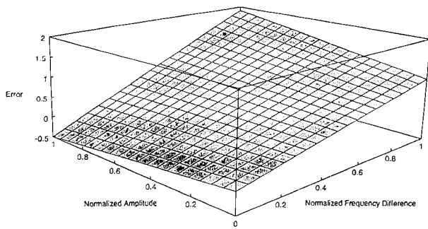
FIG. 2. An example error weighting function ( E_w ) used in the TWM procedure. The error penalty depends upon the amplitude of the measured partial normalized by the maximum amplitude partial in that frame, and the frequency difference between the measured partial frequency and the predicted harmonic frequency normalized by the measured partial frequency. For example, the best penalty (smallest error) occurs for a strong partial with small frequency difference.
