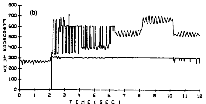
FIG. 13. Example TWM attempt for duet tracking. (a) For reference, the individual TWM results for a soprano (arpeggio with vibrato) and alto (single musical pitch) performance. (b) The TWM duet tracking results. Note the inadequate results when the two voices have similar fundamental frequencies.
