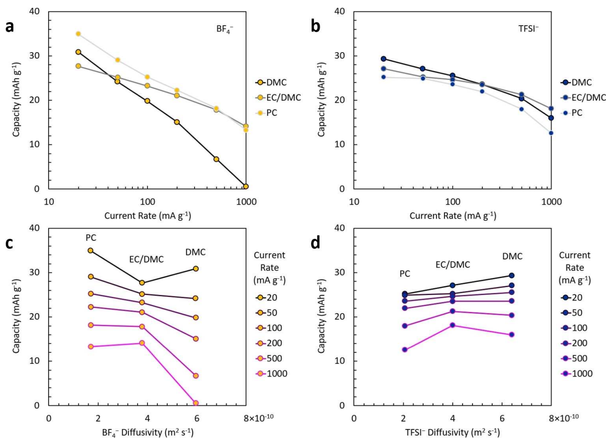
Figure 6. Anion storage capacity as a function of (a,b) current rate [mA g -1 ] and (c,d) anion diffusivity, for (a,c) BF 4 - and (b,d) TFSI - cycled between 3.0–4.0 V vs. Li/Li + .
