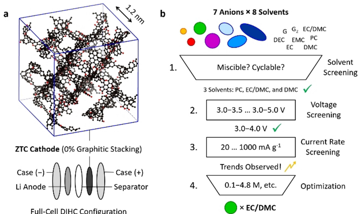
Figure 1. (a) Atomistic structural model of FAU-ZTC (Nishihara Model II + ) [20] , showing extremely high porosity ( \approx 80\% ) and no graphitic stacking, and the corresponding DIHC full-cell configuration. (b) Experimental protocol showing the field of anions and solvents screened herein, and subsequent down-selection of solvents and conditions for determining trends in capacitive ion storage in ZTC, leading to the final optimization of one anion/solvent pair.
